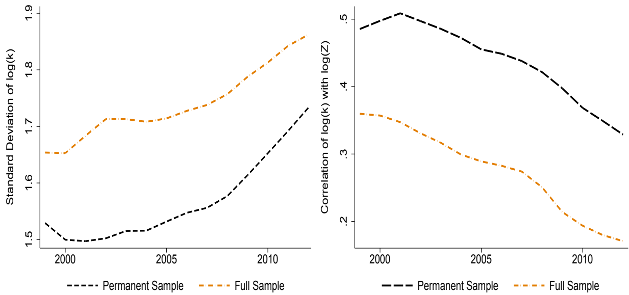
Figure VI: Log Capital Moments
